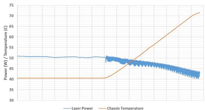
Changes in cooling system performance during steady state operation can cause power stability fluctuations and an overall drop in laser output power as shown in the chart above. The vi40 Temperature Broadcast feature can be used to sense changes in machine cooling performance and respond accordingly - before a change in application performance is noticed.
